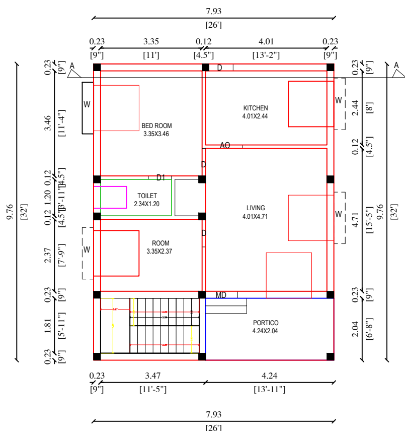
PRO.GROUND FLOOR
