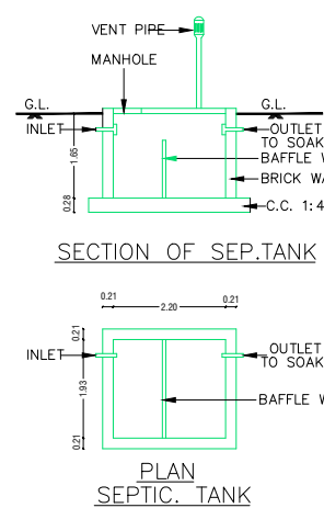
PLAN SEPTIC TANK
