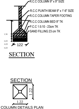
COLUMN DETAILS PLAN
