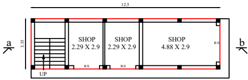
FIRST FLOOR
