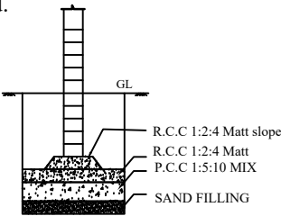
COLUMN DETAILS
