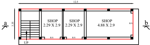
GROUND FLOOR
