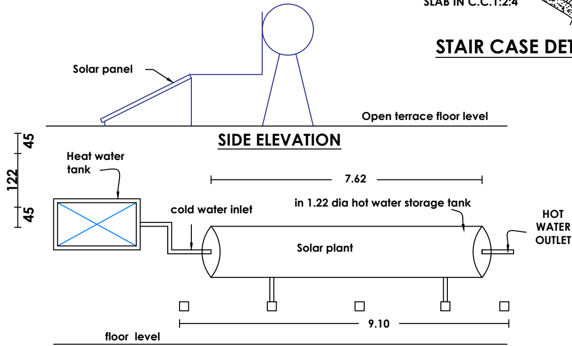
SOLAR WATER HEATER PLANT
