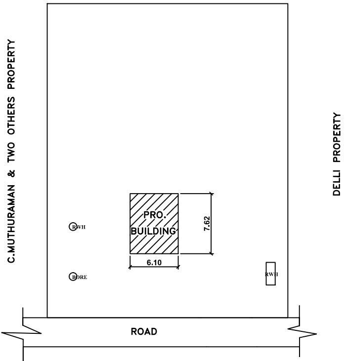
SITE PLAN
