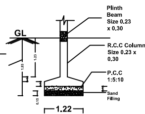
FOUNDATION DETAILS
