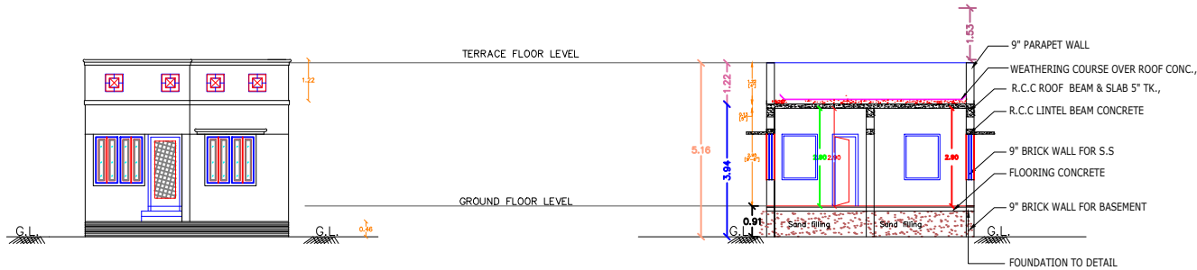
FRONT ELEVATION
