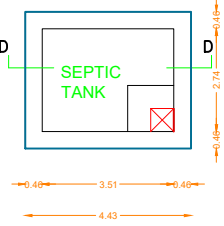
PLAN OF SEPTIC TANK
