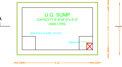
SUMP DETAIL SCALE 1"=4'-0"
