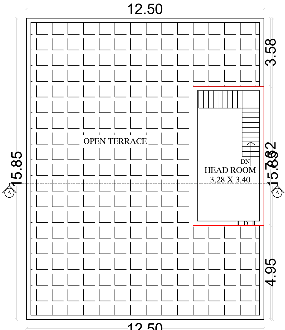
PROPOSED FIRST FLOOR HEAD ROOM PLAN
