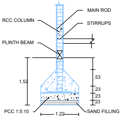
COLUMN DETAILS
