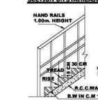
SECTION ON STAIRCASE
