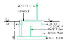
SECTION OF SEPT. TANK
