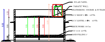
CUT SECTION ON AA
