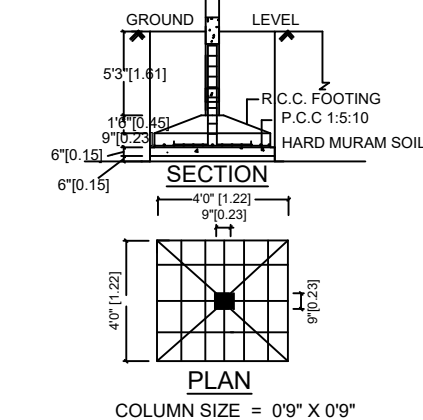
FOUNDATION DETAILS
