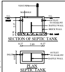
PLAN SEPTIC TANK
