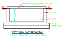
RWH SECTION (SAMPLE) RWH CAPACITY : 1 - 5000 LTRS
