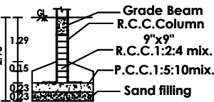
COLUMN DETAILS
