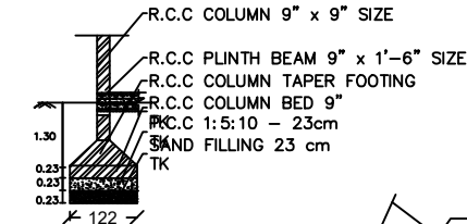
SECTION COLUMN DETAILS PLAN
