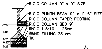
COLUMN DETAILS PLAN
