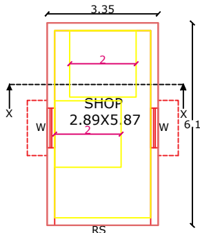
PROPOSED SHOP PLAN
