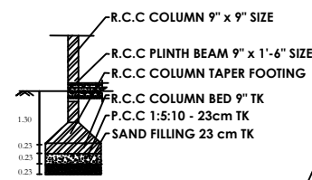
COLUMN DETAILS PLAN
