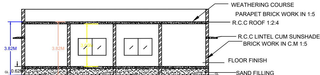
SECTION ON XX
