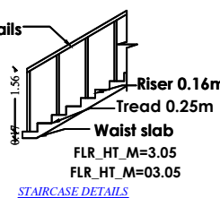
STAIRCASE DETAILS
