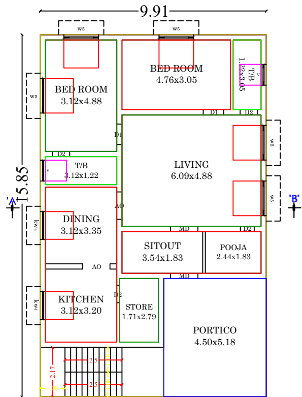
BLOCK I - FLOOR 0 GROUND FLOOR PLAN
