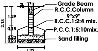
COLUMN DETAILS
