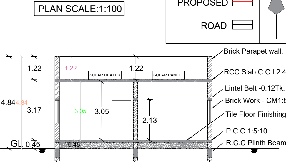
CROSS SECTION-CS
