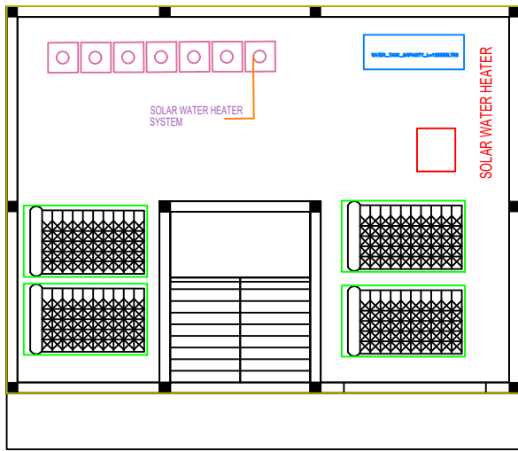
PROPOSED TERRACED FLOOR
