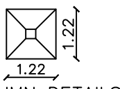
COLUMN DETAILS PLAN
