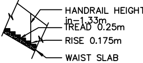
STAIRCASE DETAILS
