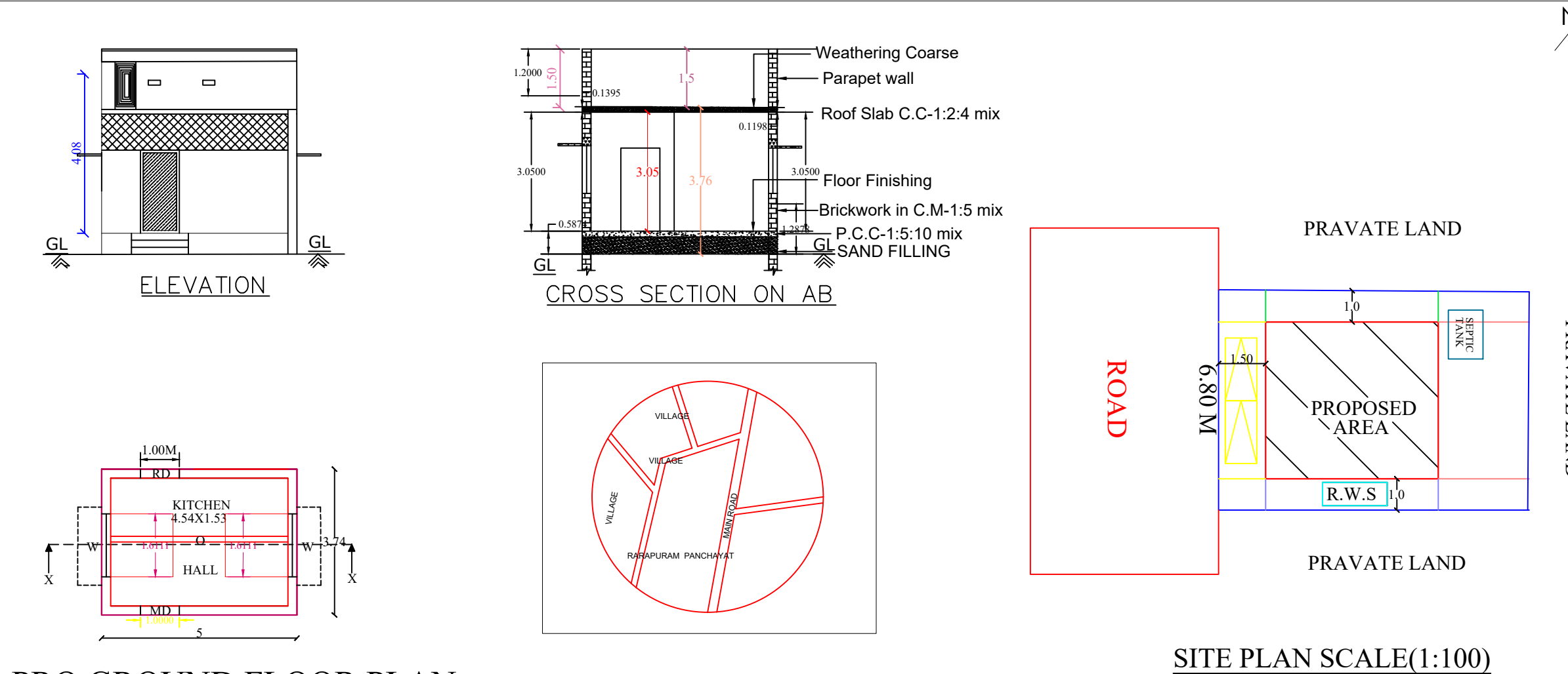
PROPOSED FLOOR PLAN
