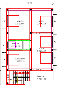
FLOOR PLAN
