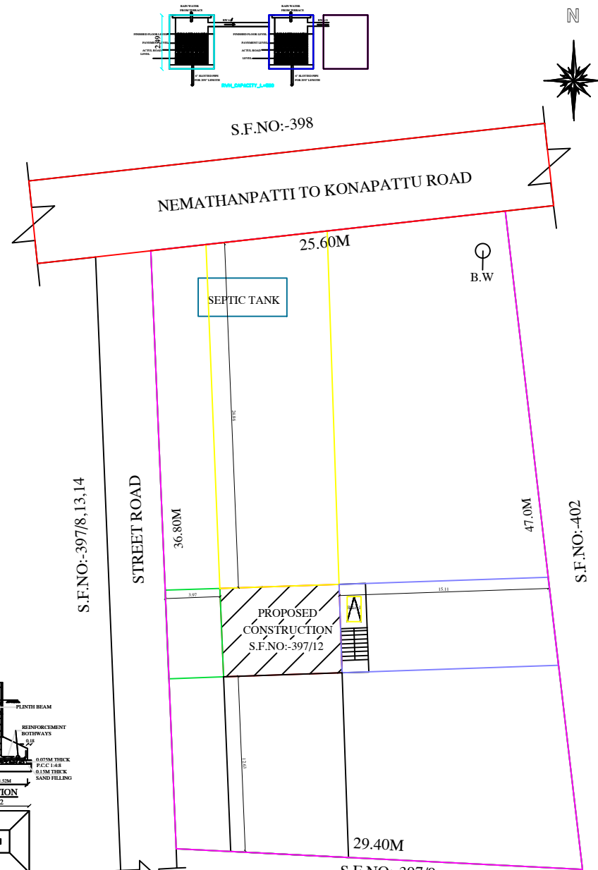
SITE PLAN
