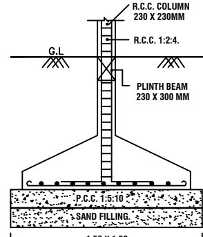
FOUNDATION DETAIL
