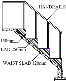
STAIRCASE DETAILS
