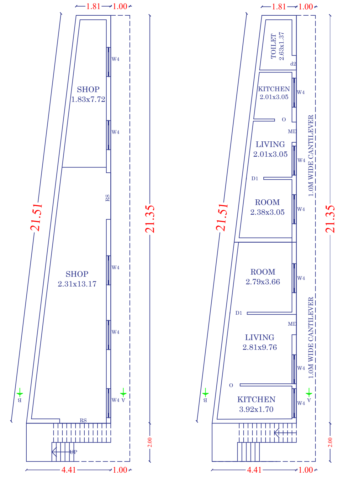
GROUND FLOOR PLAN COMMERCIAL BUILDING FIRST FLOOR PLAN RESIDENTIAL BUILDING
