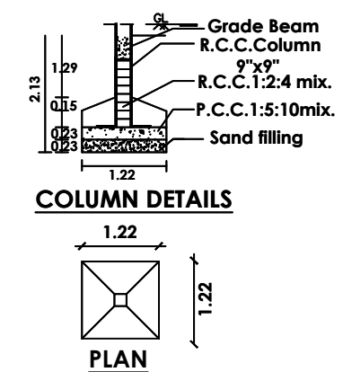
COLUMN DETAILS
