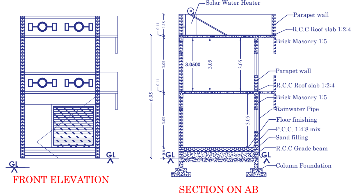
FRONT ELEVATION SECTION ON AB
