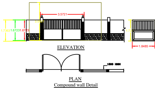
PLAN Compound wall Detail
