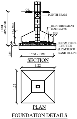
FOUNDATION DETAILS
