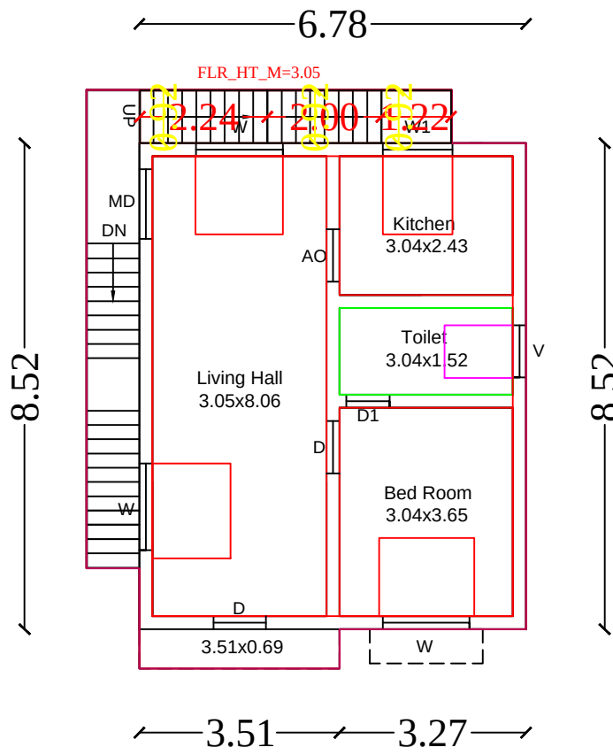
Propose First Floor
