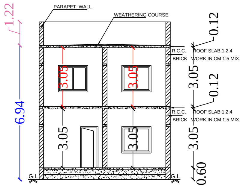
Section on-"AA"
