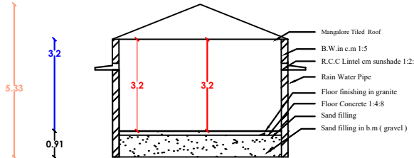
SECTION "PB"
