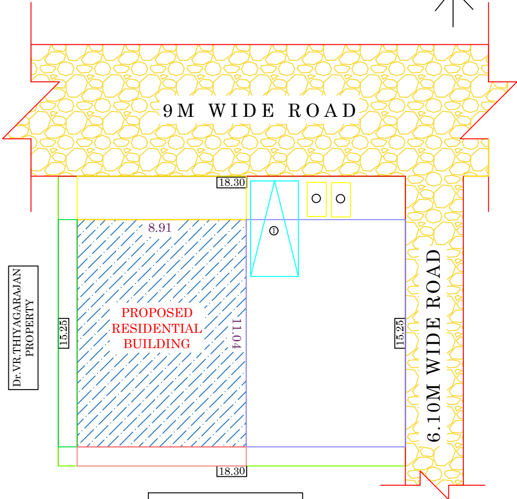
SITE PLAN
