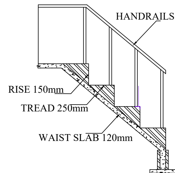
STAIRCASE DETAILS
