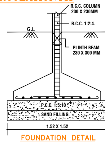
FOUNDATION DETAIL
