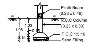
FOUNDATION DETAILS ( Scale 1:100 )
