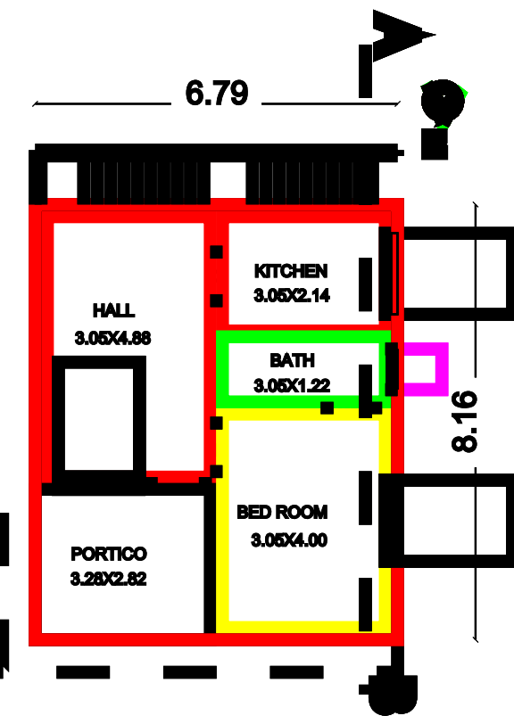
PROPOSED GROUND
