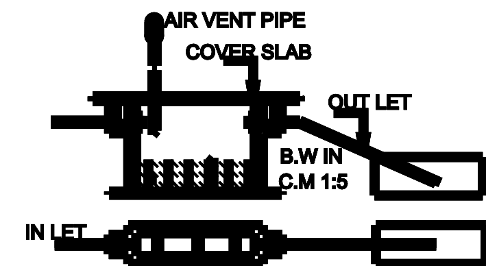
DETAILS OF SEPTIC TANK & D-TRENCH
