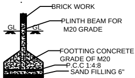
FOOTING DETAILS
