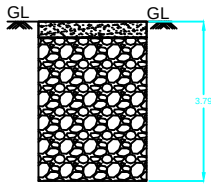
RWH SECTION
