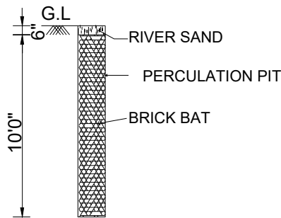
PERCOLATION PIT
