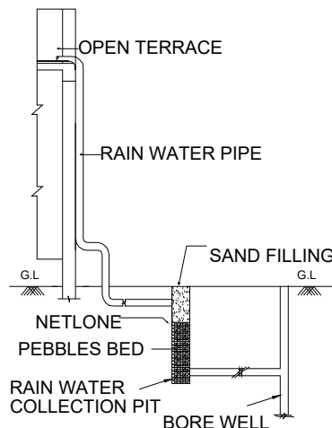
RAIN WATER
