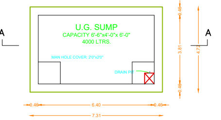
SUMP DETAIL SCALE 1"=4'0"
