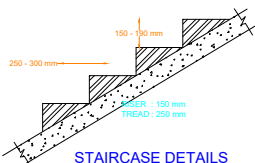
STAIRCASE DETAILS NOT TO SCALE
