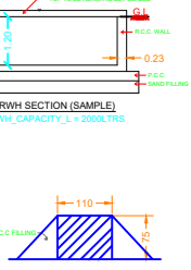
DWARF WALL SECTION NOT TO SCALE
