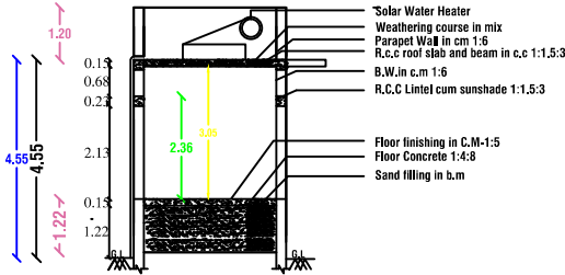
SECTION - "AB "
