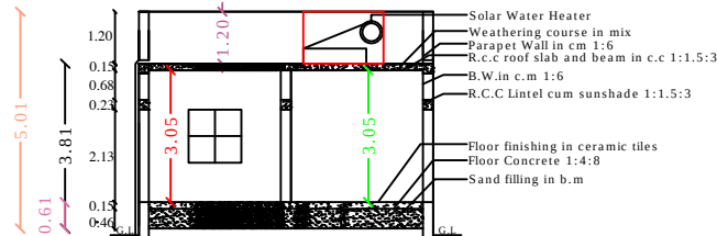
SECTION - "AB "
