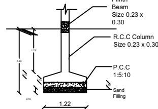
FOUNDATION DETAILS
