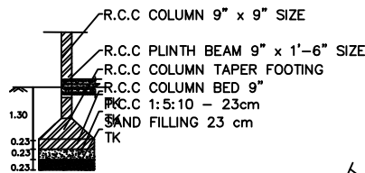
SECTION
