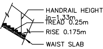
STAIRCASE DETAILS
