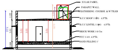
CUT SECTION ON AA
