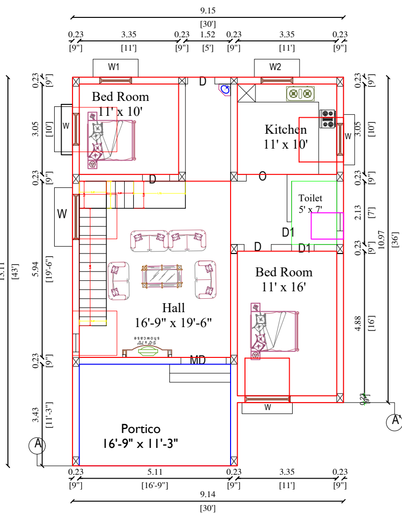
PRO.GROUND FLOOR
