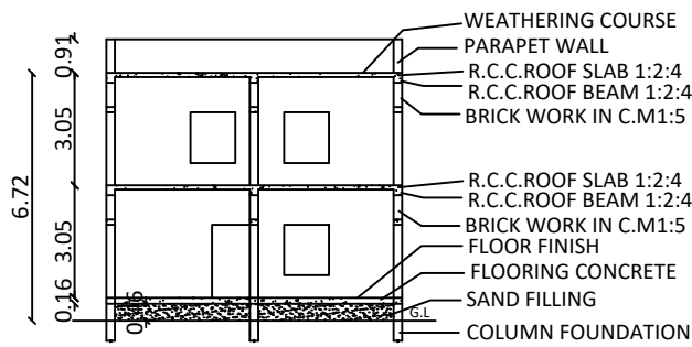
SECTION-SS
