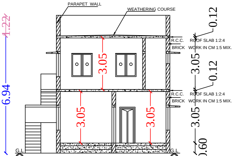
Section on-AA
