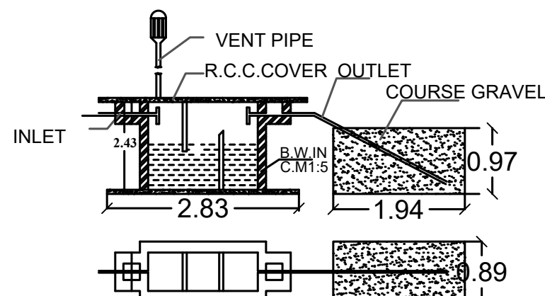
SEPTIC TANK & D-TRENCH DETAILS NOT TO SCALE
