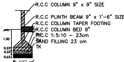
SECTION
