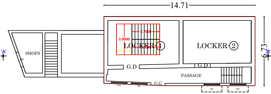
FLOOR 0 EXISTINTG GROUND FLOOR PLAN
