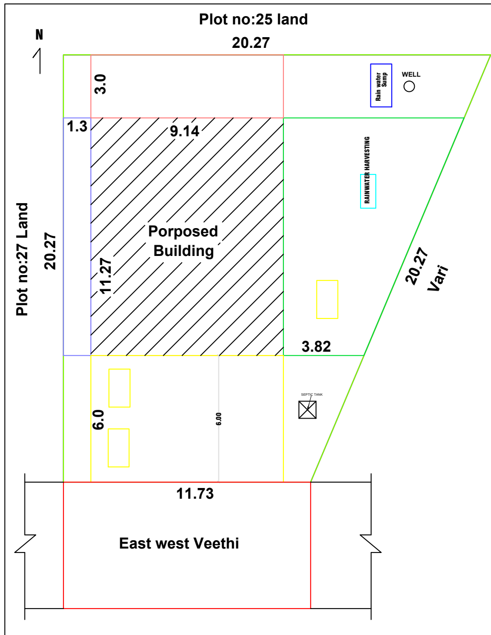
SITE PLAN CUM KEYPLAN
