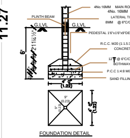
FOUNDATION DETAILS
