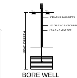
BORE WELL
