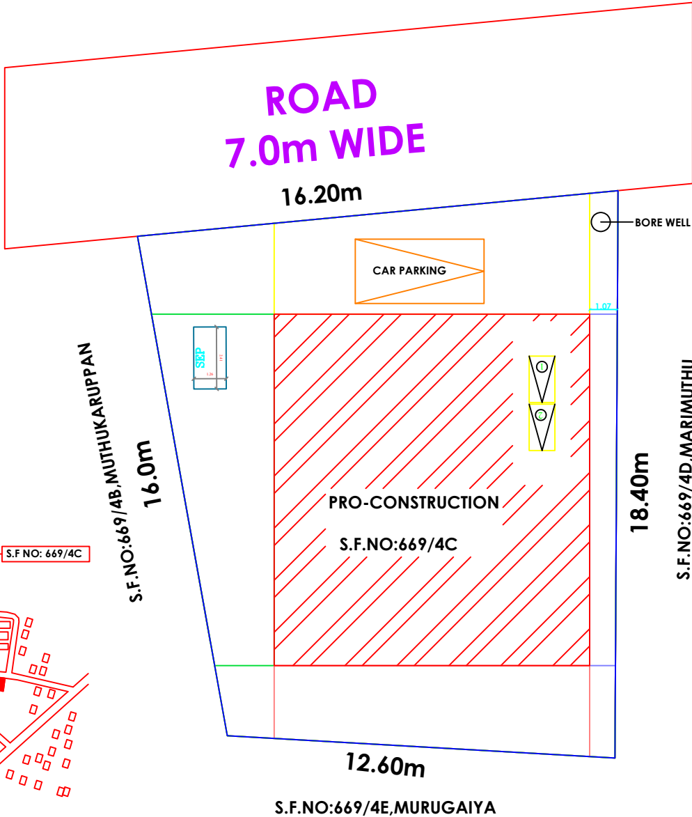
TOPO PLAN
