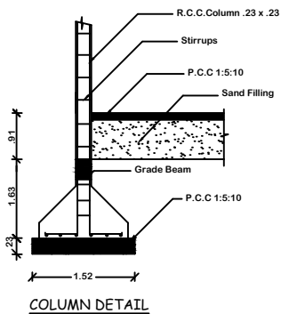
COLUMN DETAIL
