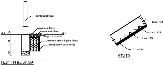
PLINTH BOUNDARY
