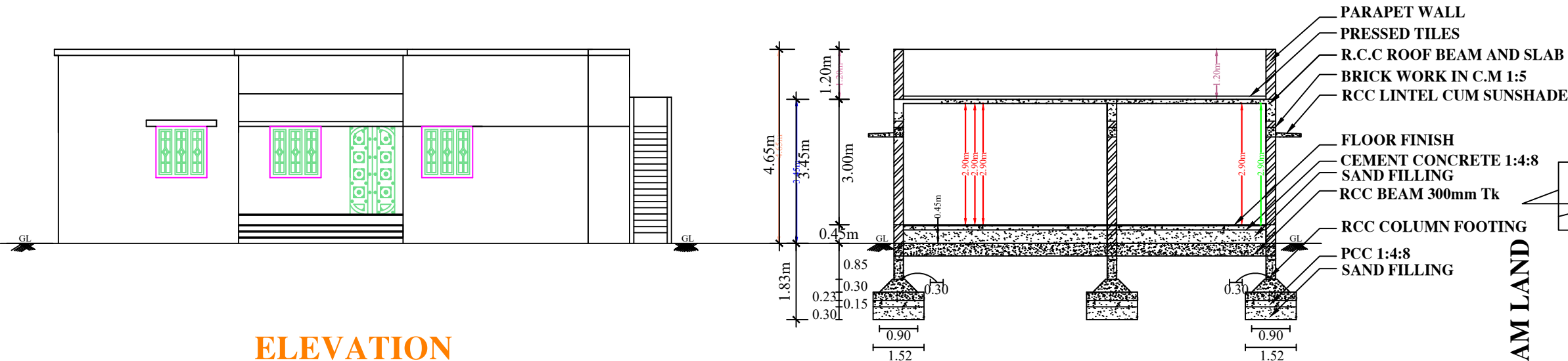
SECTION [A-A]
