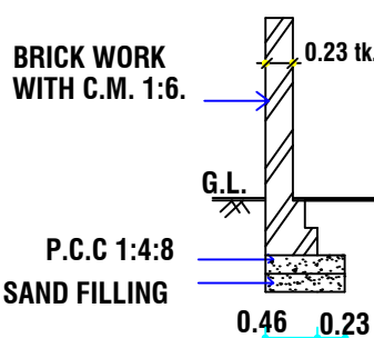
SECTION OF COMPOUND WALL
