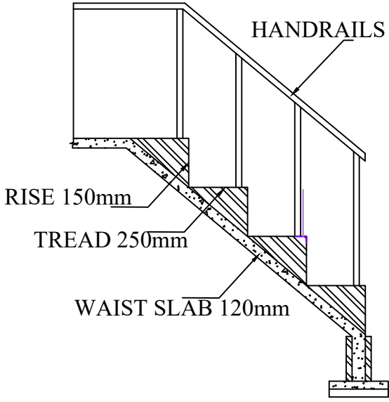
STAIRCASE DETAILS
