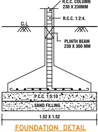
FOUNDATION DETAIL
